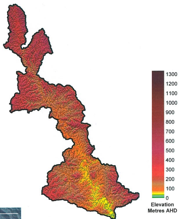
Catchment Elevation
