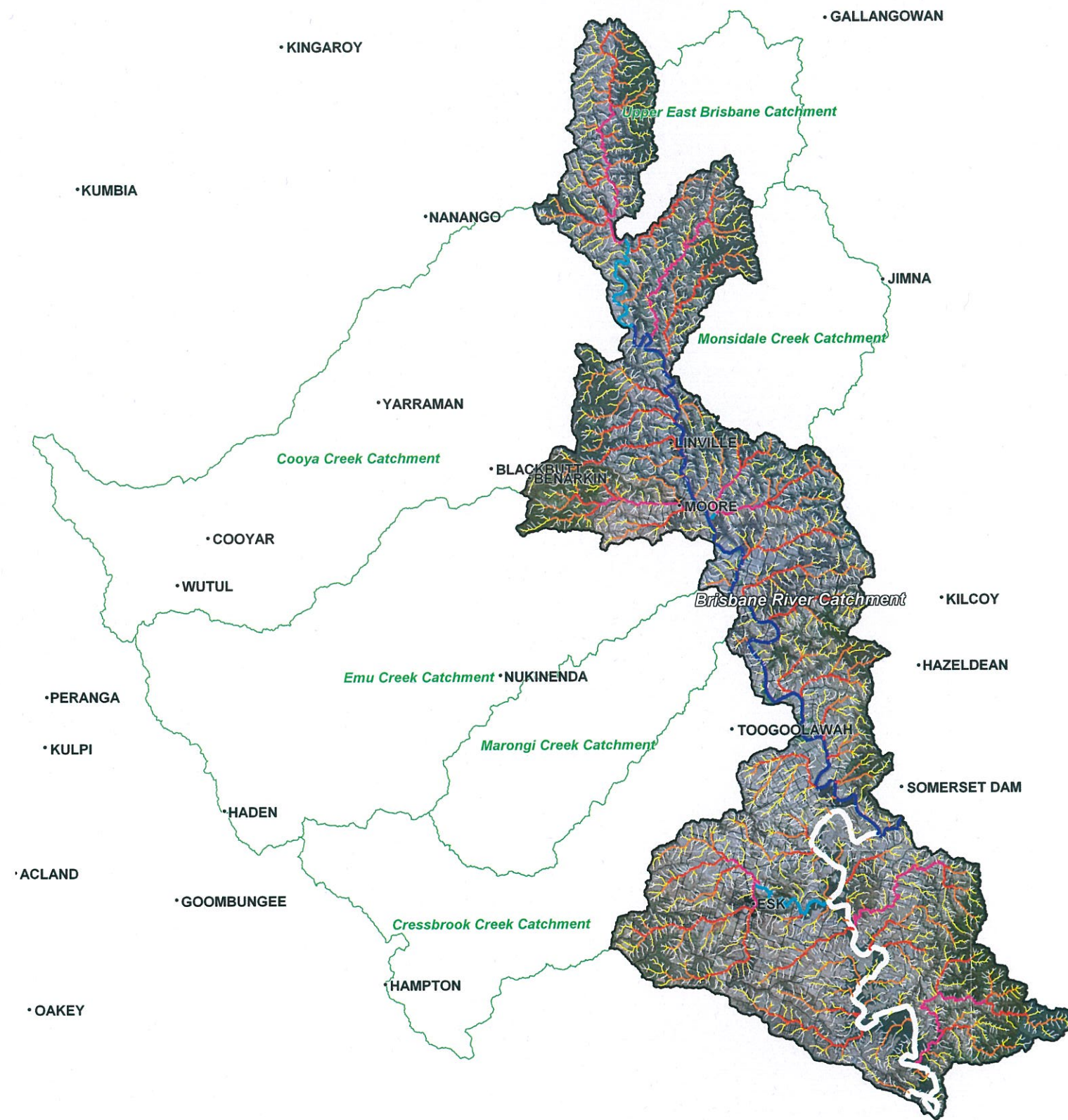
Stream Order
